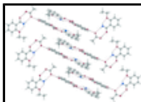
Fig. 3. Section of the crystal structure, showing the \pi - \pi stacking interaction between the aromatic rings of the four-component molecular assemblies.
